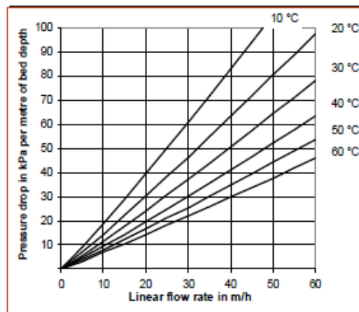
Figure 2 : Pressure Drop
